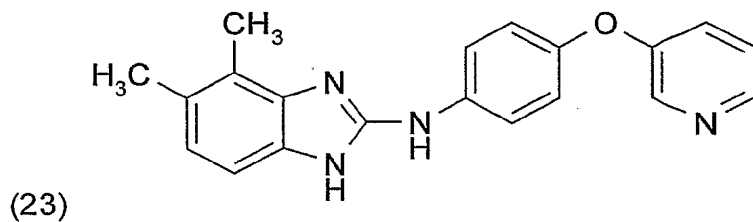
(4,5-Dimethyl-1H-benzimidazol-2-yl)-[4-(pyridin-3-yloxy)-phenyl]-amin
